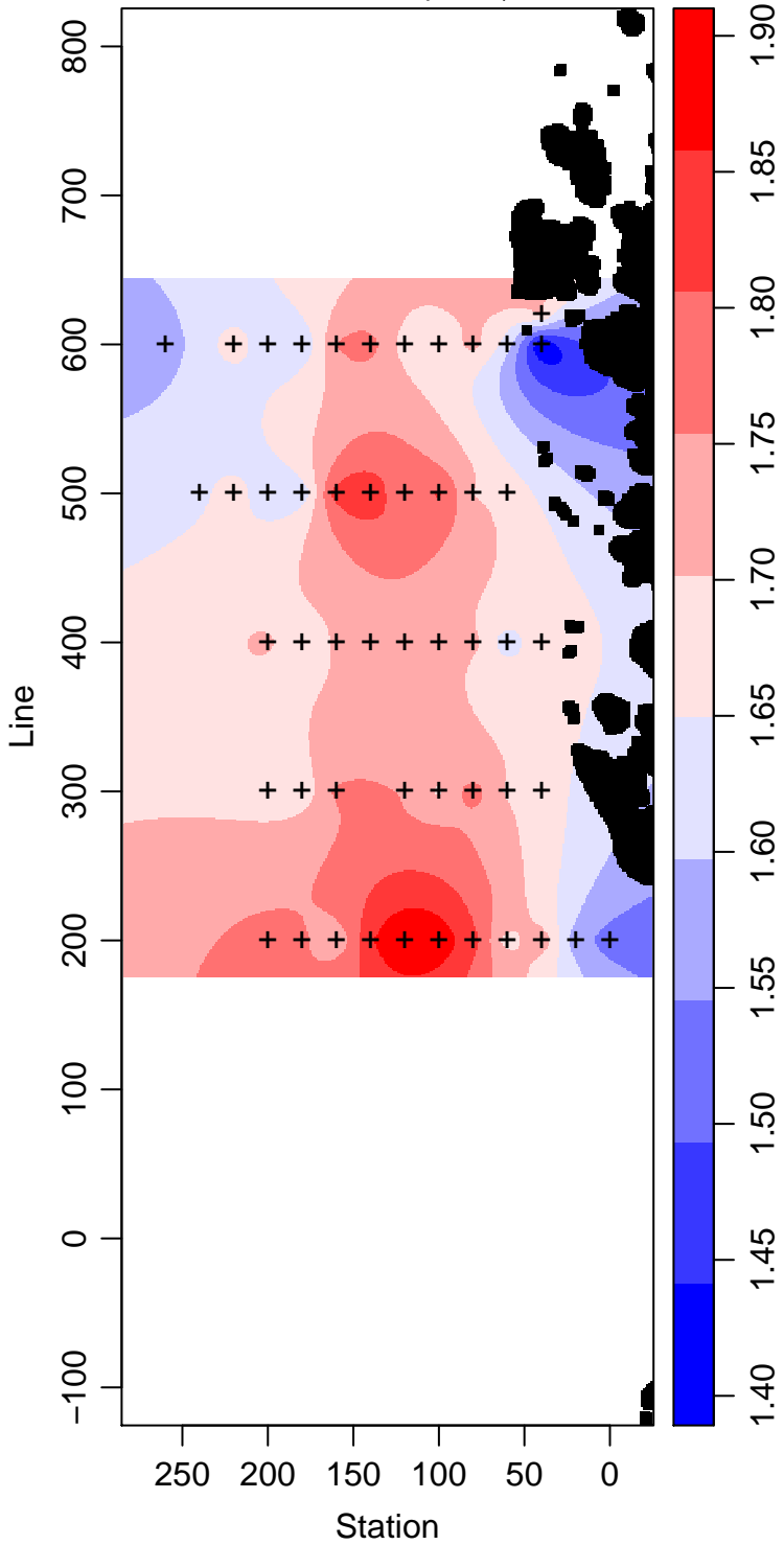
LMG03-01_60_Phosphate \mu\text{ mol L}^{-1}
