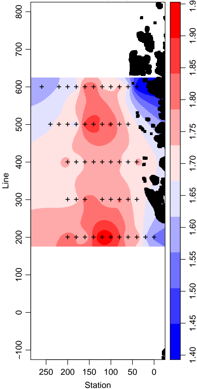
LMG03-01_65_Phosphate \mu\text{ mol L}^{-1}
