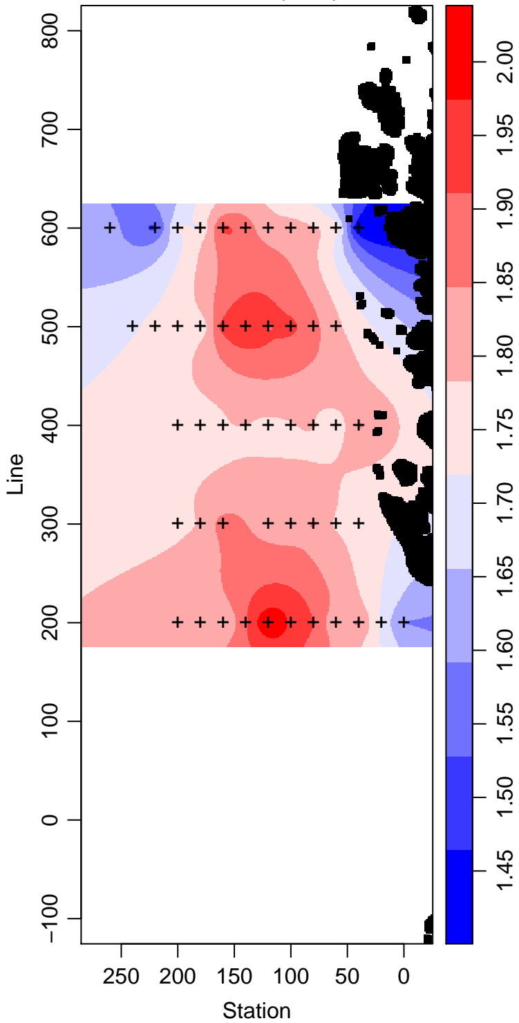
LMG03-01_75_Phosphate \mu\text{ mol L}^{-1}
