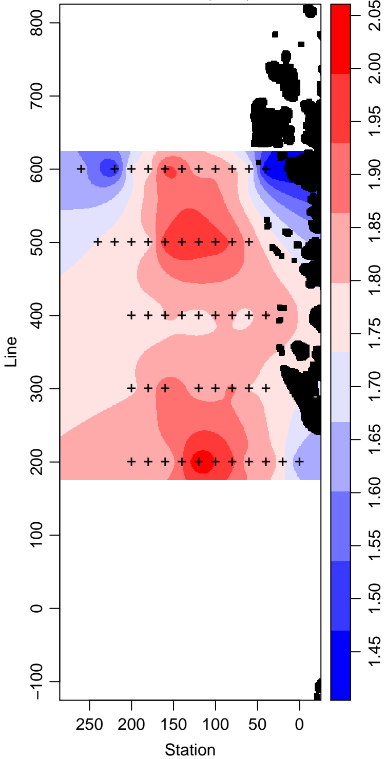
LMG03-01_80_Phosphate \mu\text{ mol L}^{-1}
