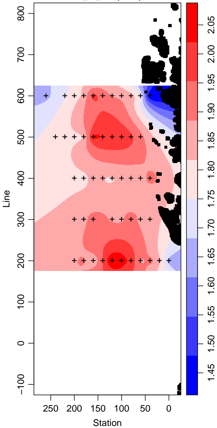
LMG03-01_90_Phosphate \mu\text{ mol L}^{-1}
