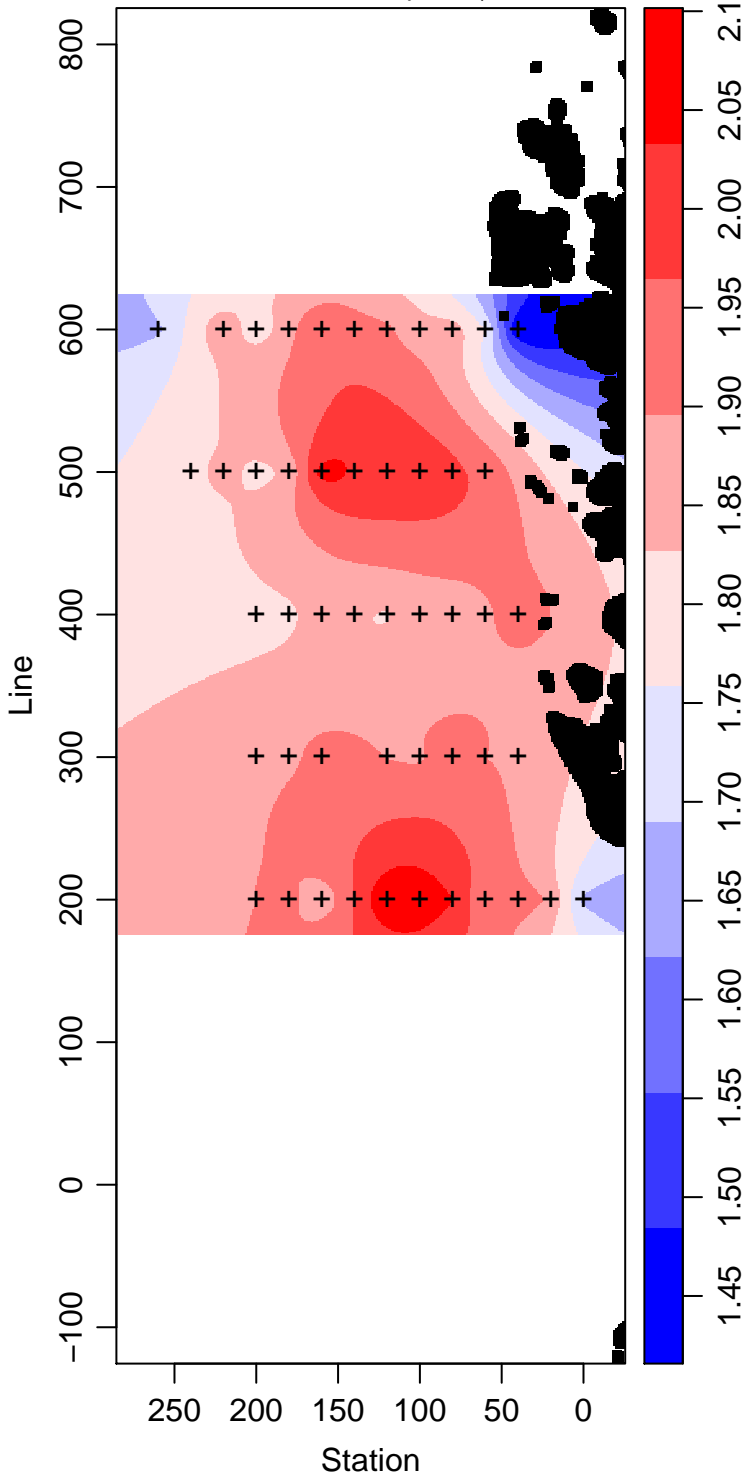
LMG03-01_95_Phosphate \mu\text{ mol L}^{-1}
