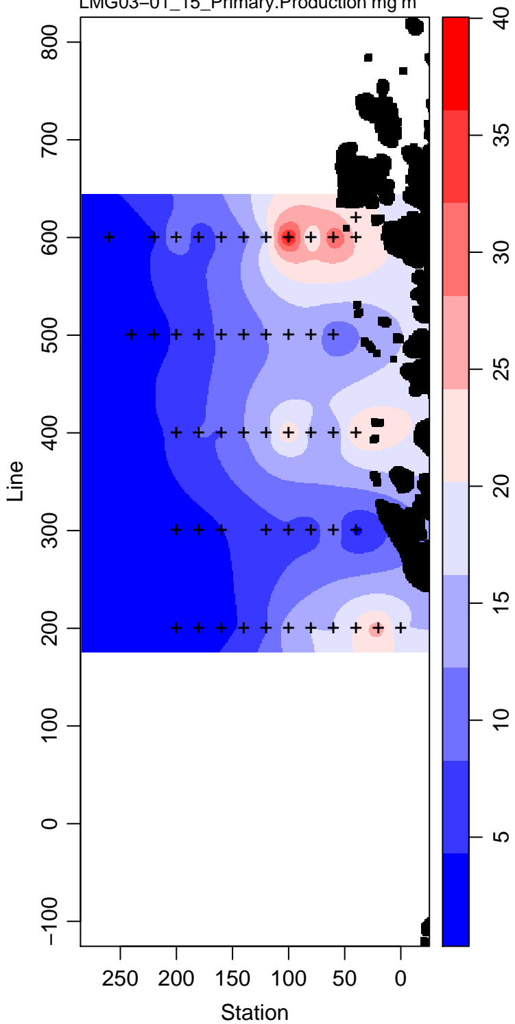
LMG03-01_15_Primary.Production mg m -3
