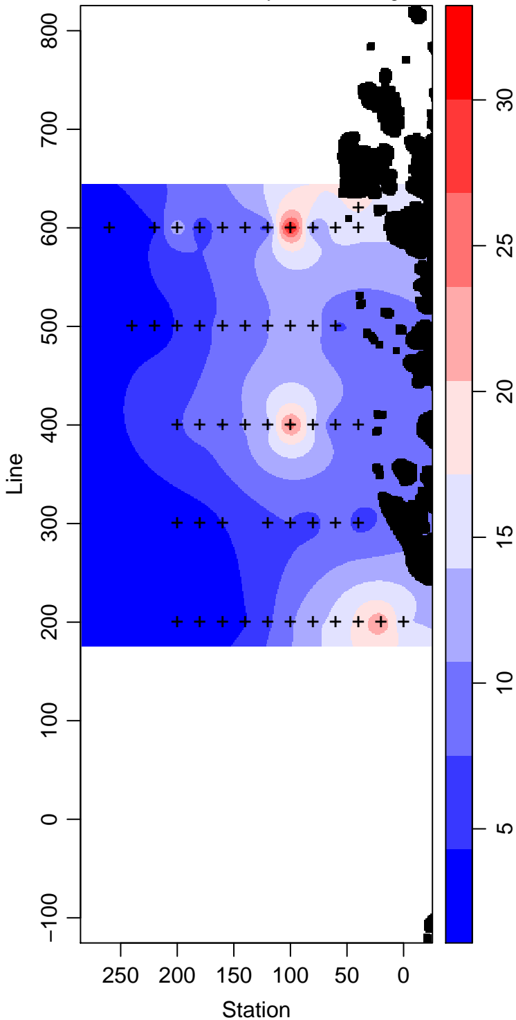
LMG03-01_20_Primary.Production mg m -3
