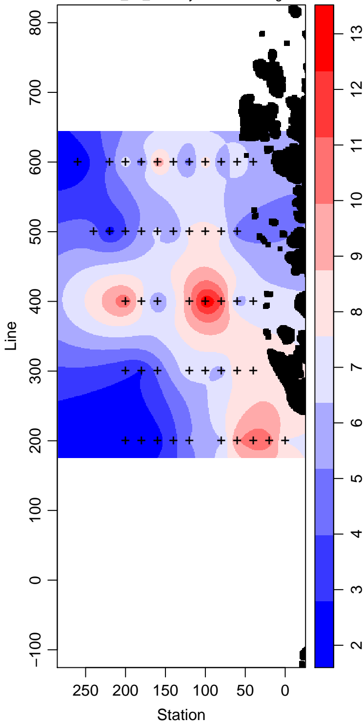
LMG03-01_30_Primary.Production mg m -3
