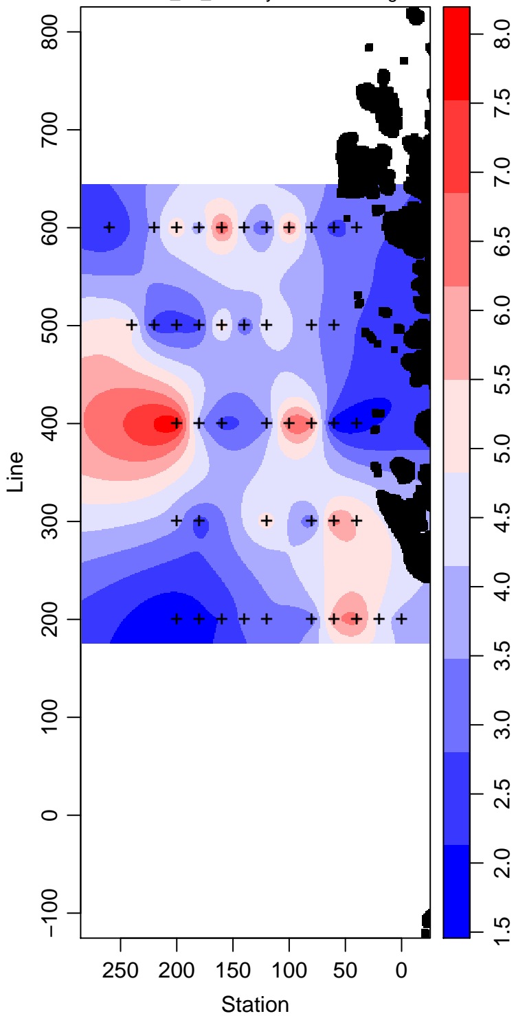
LMG03-01_45_Primary.Production mg m -3
