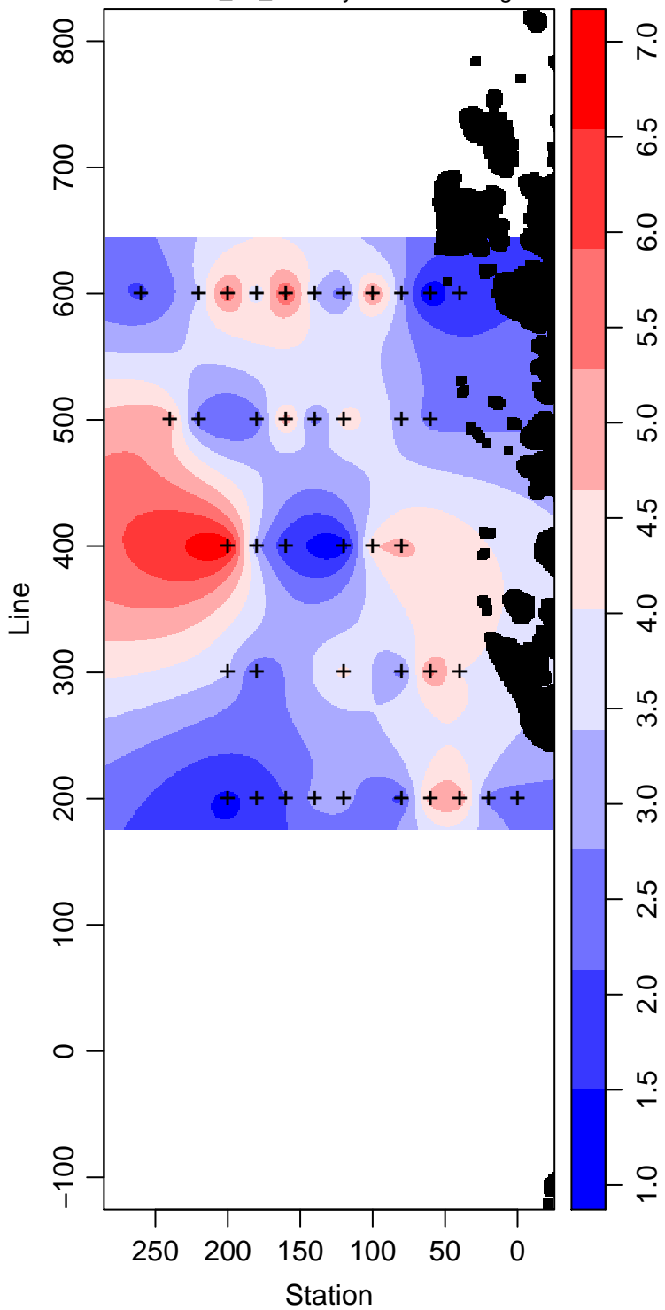
LMG03-01_50_Primary.Production mg m -3
