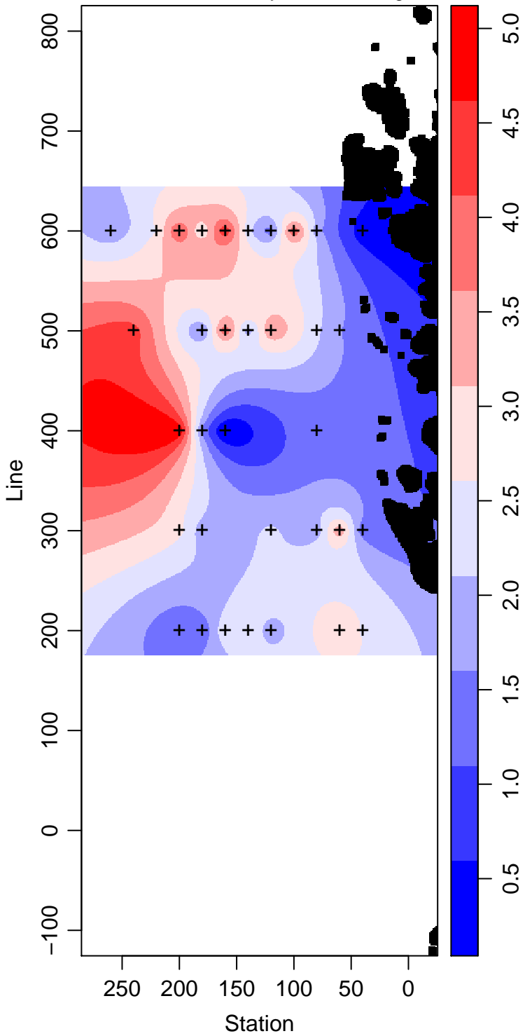
LMG03-01_60_Primary.Production mg m -3
