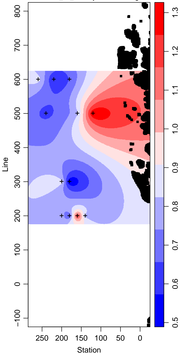
LMG03-01_90_Primary.Production mg m -3
