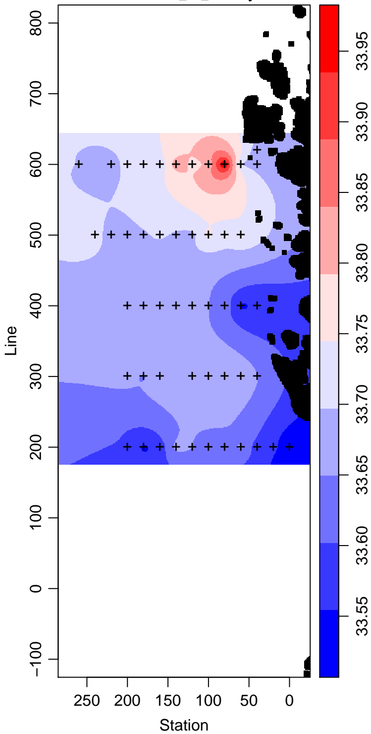
LMG03-01_20_Salinity
