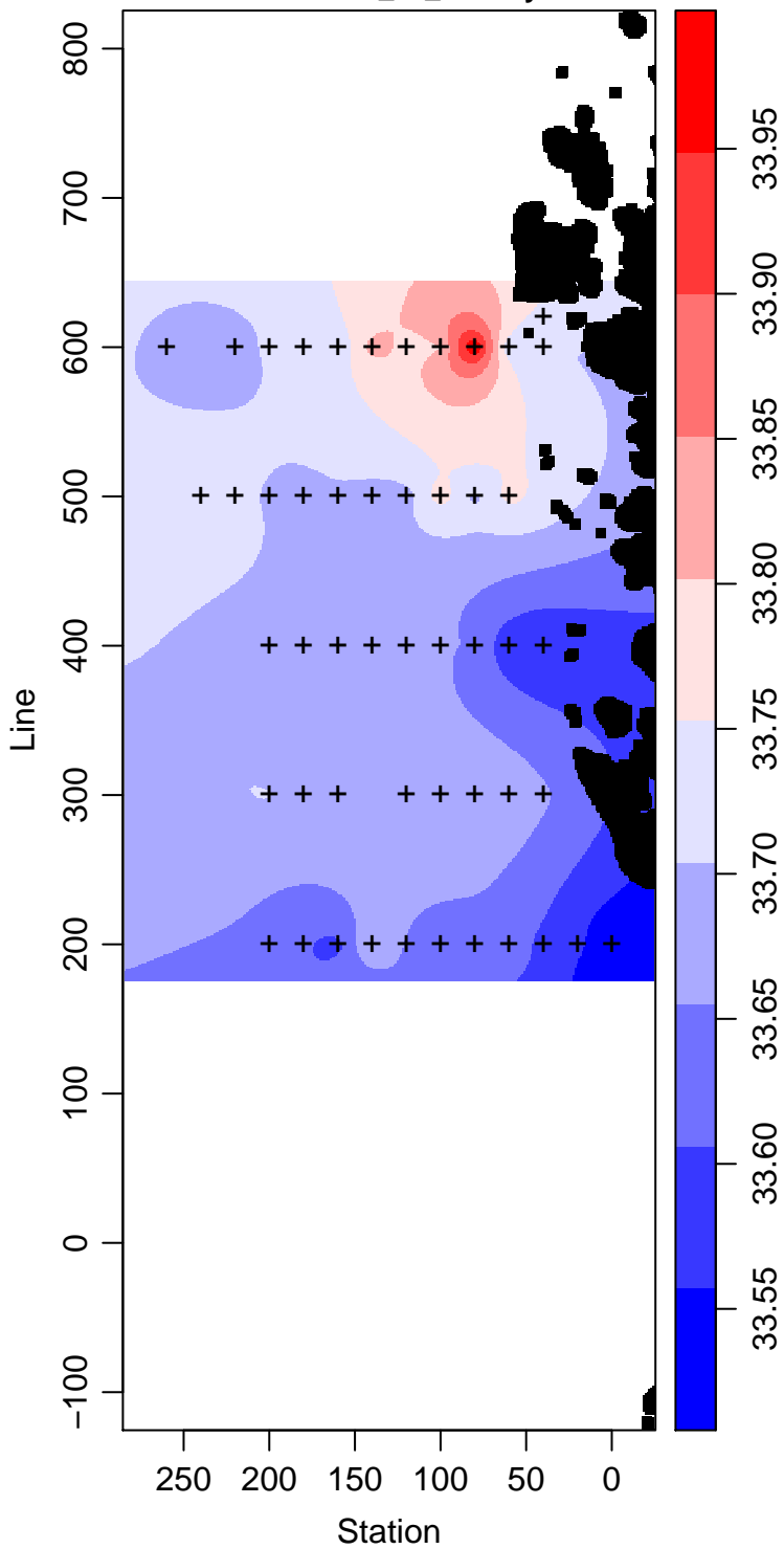
LMG03-01_25_Salinity
