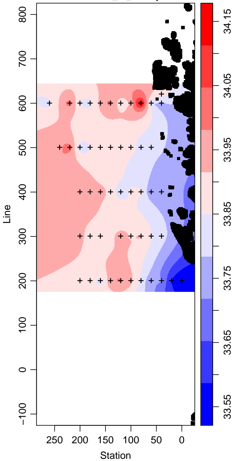
LMG03-01_55_Salinity
