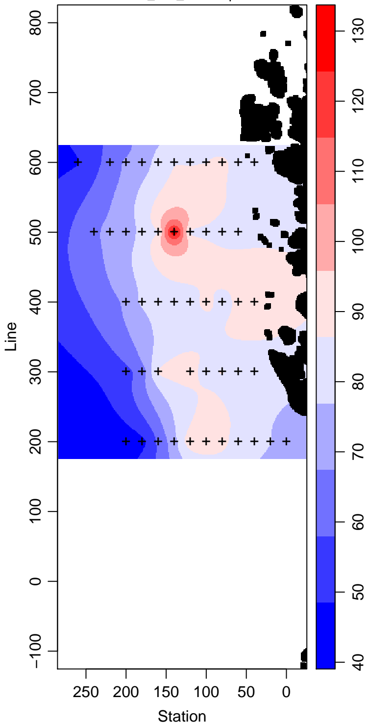
LMG03-01_100_Silicate \mu\text{ mol L}^{-1}
