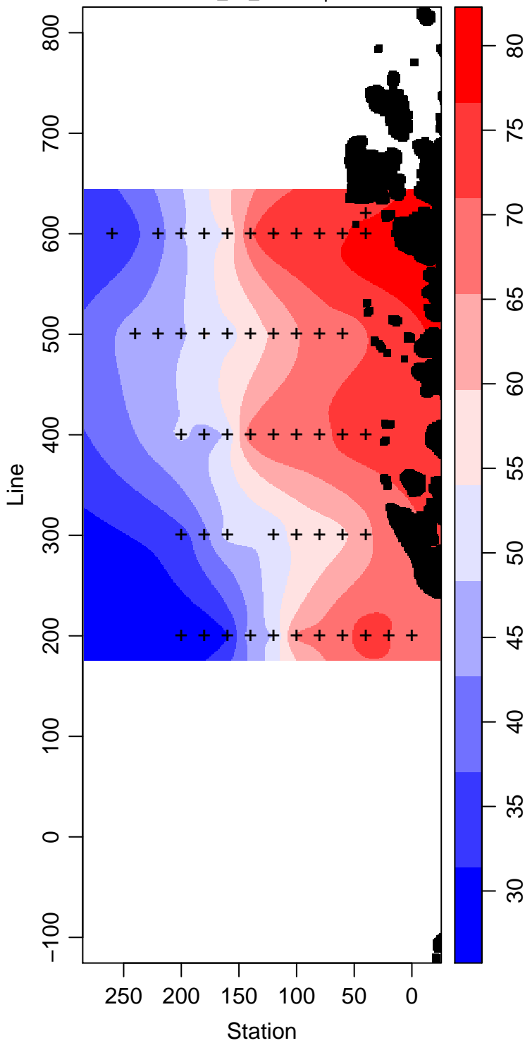
LMG03-01_20_Silicate \mu\text{ mol L}^{-1}
