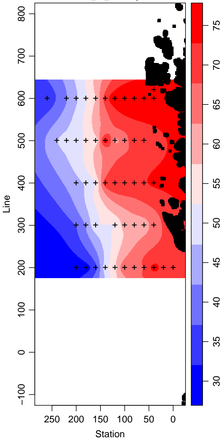
LMG03-01_30_Silicate \mu\text{ mol L}^{-1}
