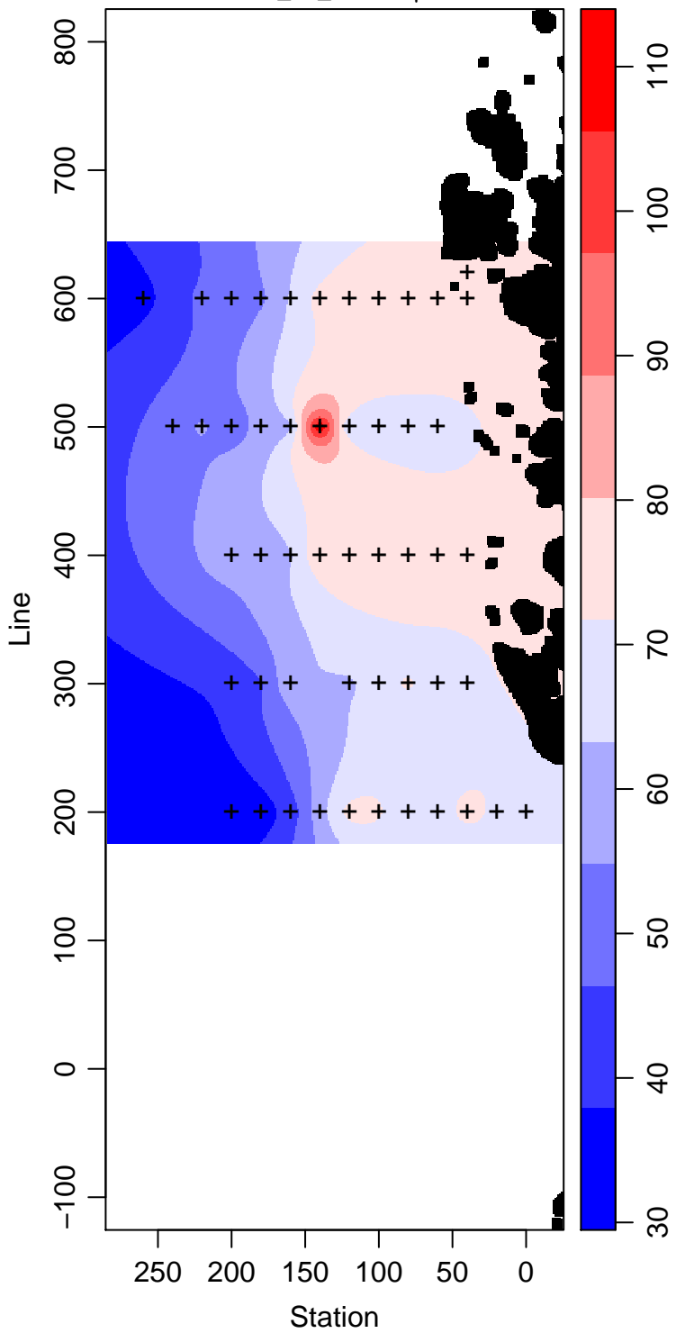
LMG03-01_45_Silicate \mu\text{ mol L}^{-1}
