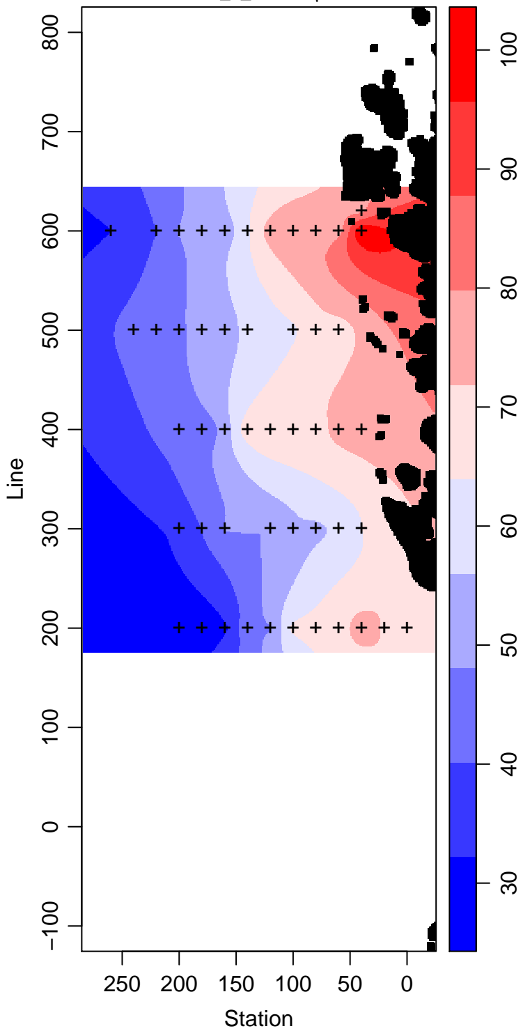
LMG03-01_5_Silicate \mu\text{ mol L}^{-1}
