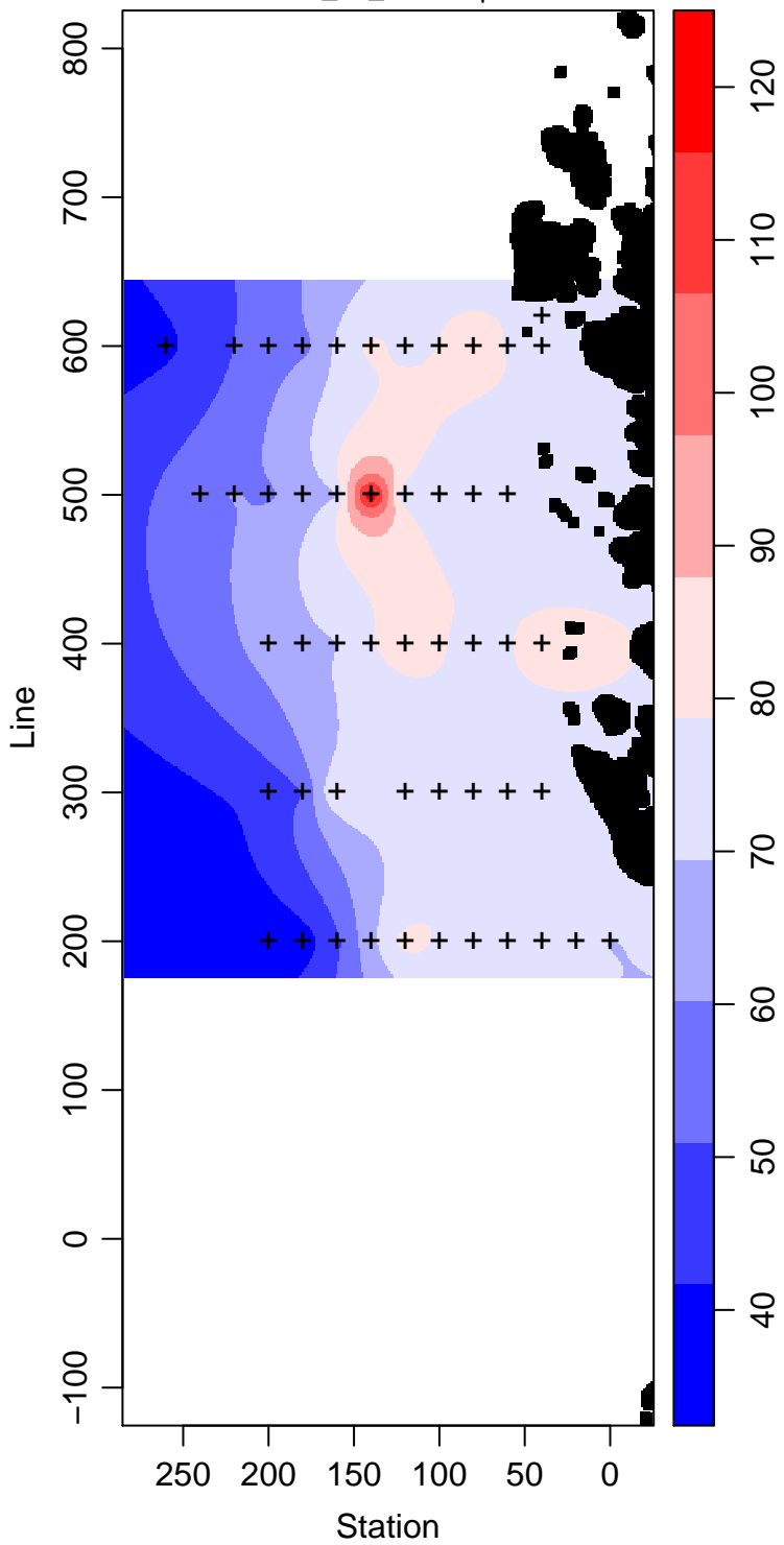
LMG03-01_60_Silicate \mu\text{ mol L}^{-1}
