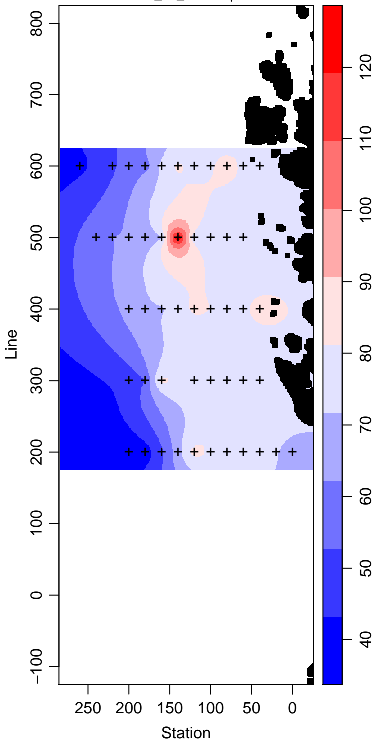
LMG03-01_65_Silicate \mu\text{ mol L}^{-1}
