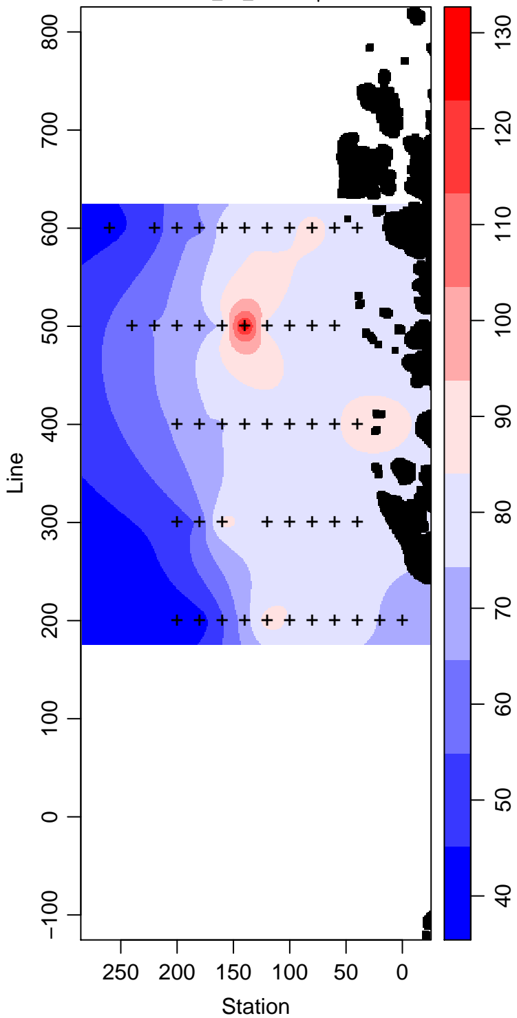
LMG03-01_75_Silicate \mu\text{ mol L}^{-1}
