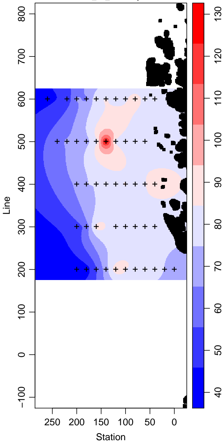
LMG03-01_80_Silicate \mu\text{ mol L}^{-1}
