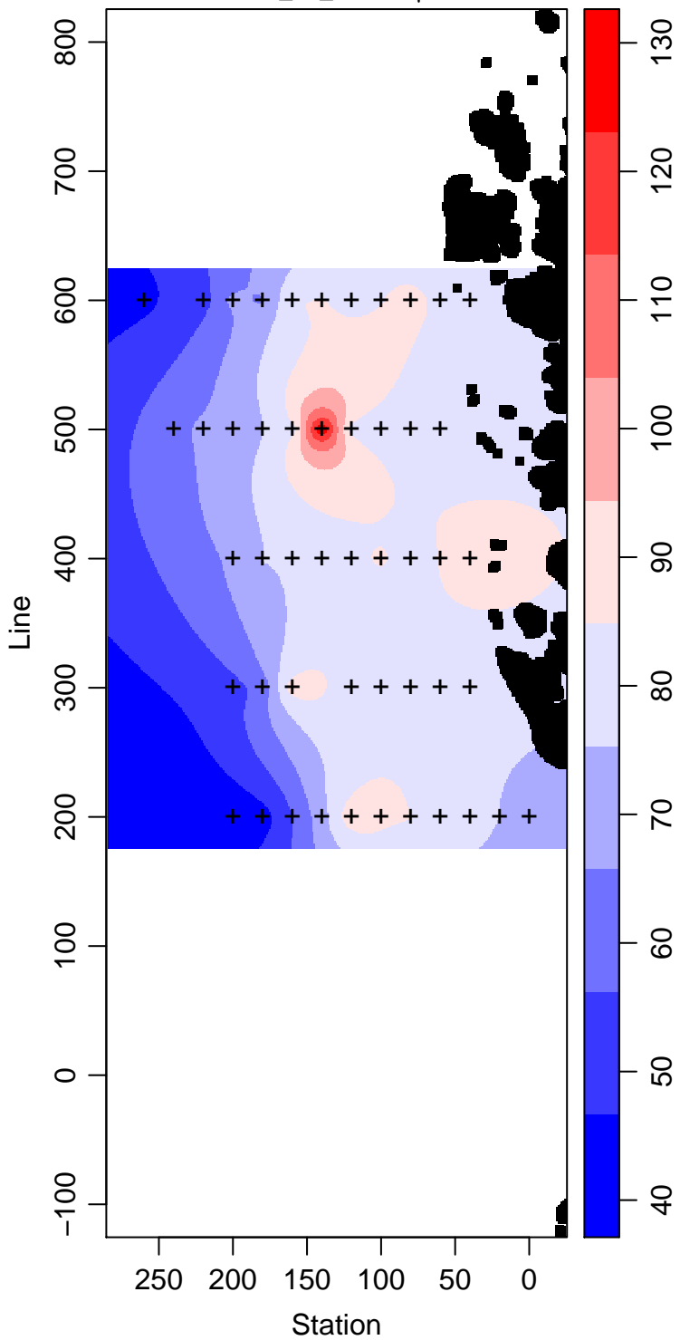
LMG03-01_85_Silicate \mu\text{ mol L}^{-1}
