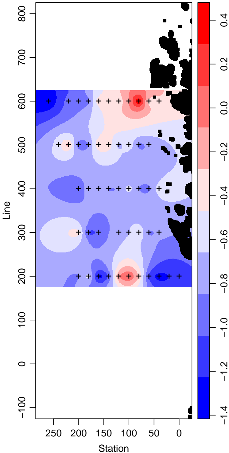
LMG03-01_100_Temperature ° Celsius
