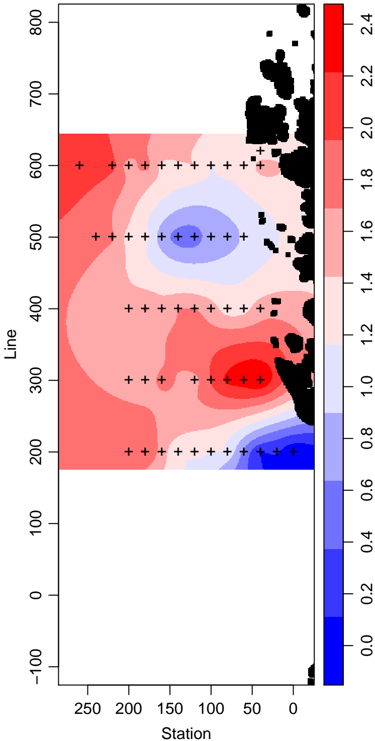
LMG03-01_1_Temperature ° Celsius
