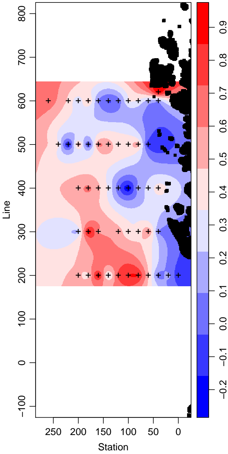
LMG03-01_30_Temperature ° Celsius
