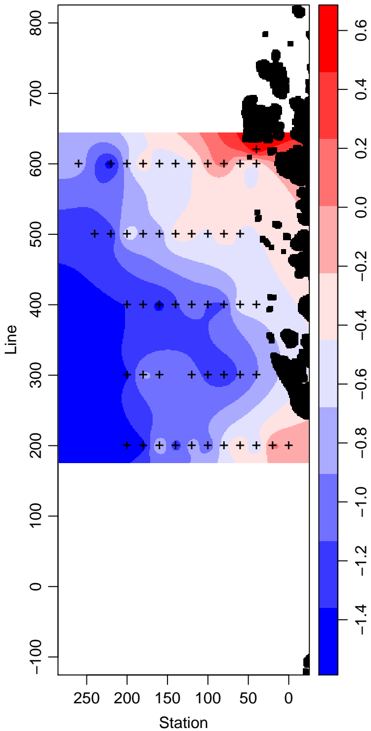
LMG03-01_55_Temperature ° Celsius
