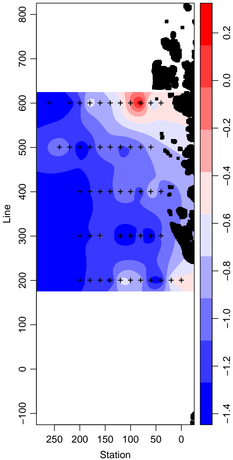
LMG03-01_75_Temperature ° Celsius
