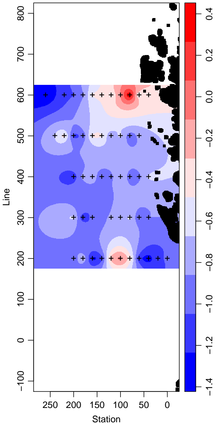
LMG03-01_95_Temperature ° Celsius
