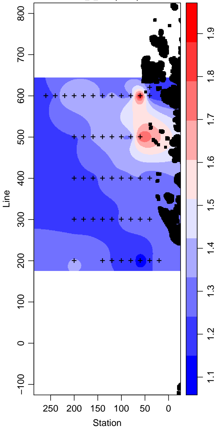
LMG04-01_1_Phosphate \mu\text{ mol L}^{-1}
