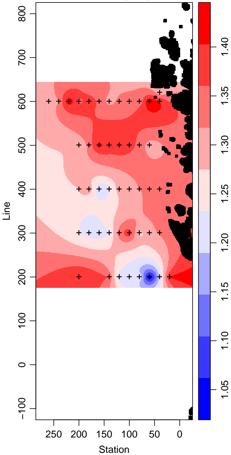
LMG04-01_25_Phosphate \mu\text{ mol L}^{-1}
