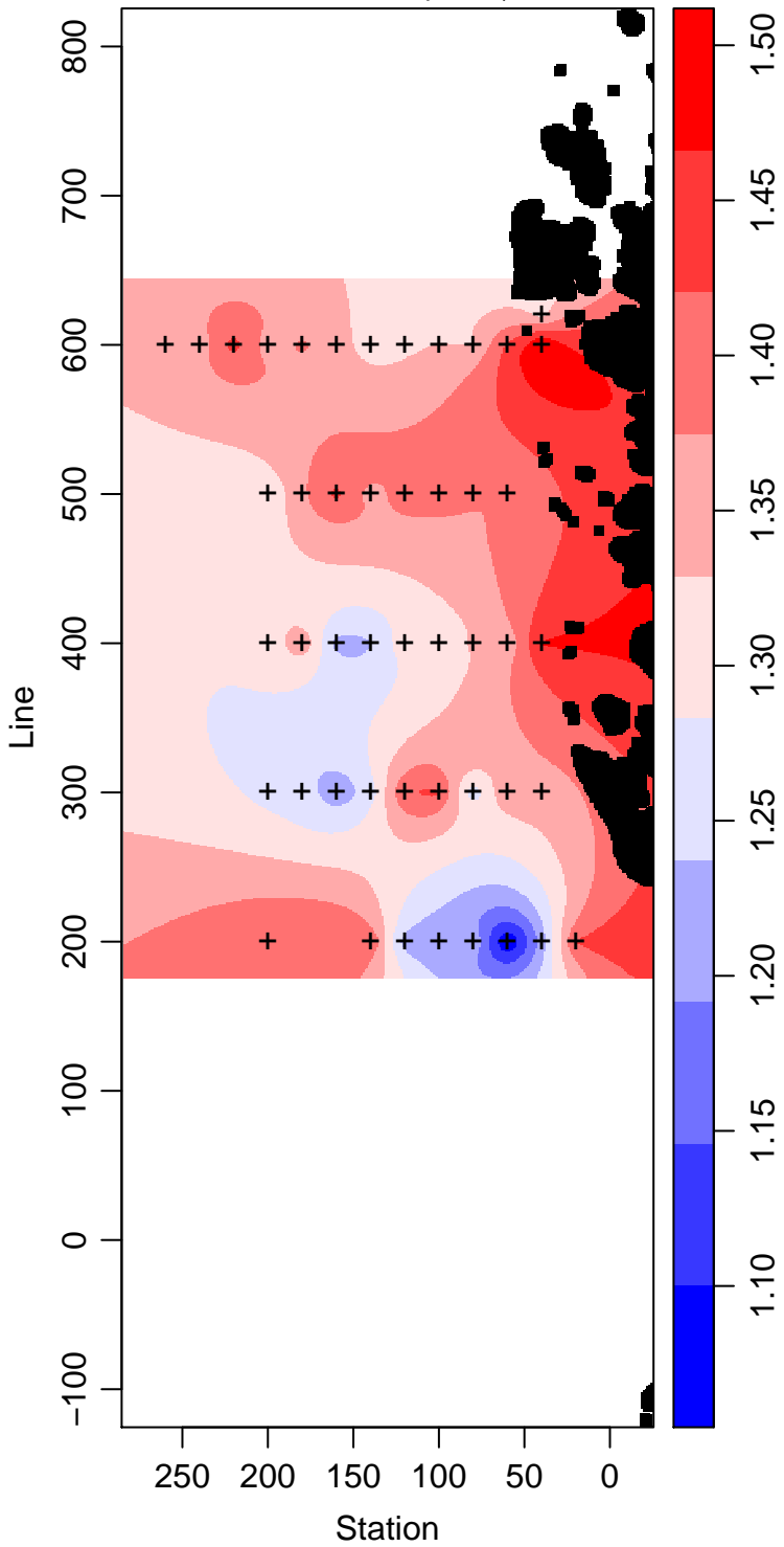
LMG04-01_30_Phosphate \mu\text{ mol L}^{-1}
