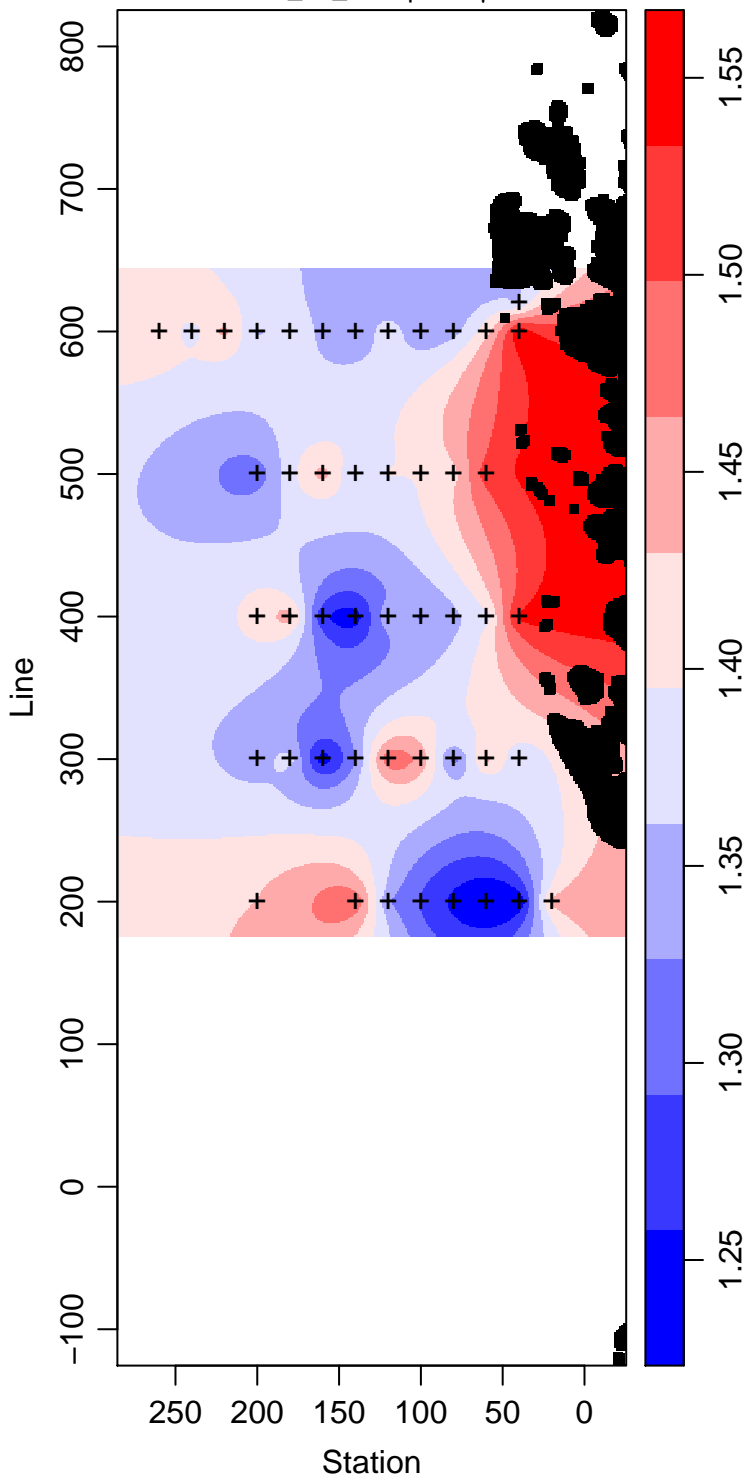
LMG04-01_35_Phosphate \mu\text{ mol L}^{-1}
