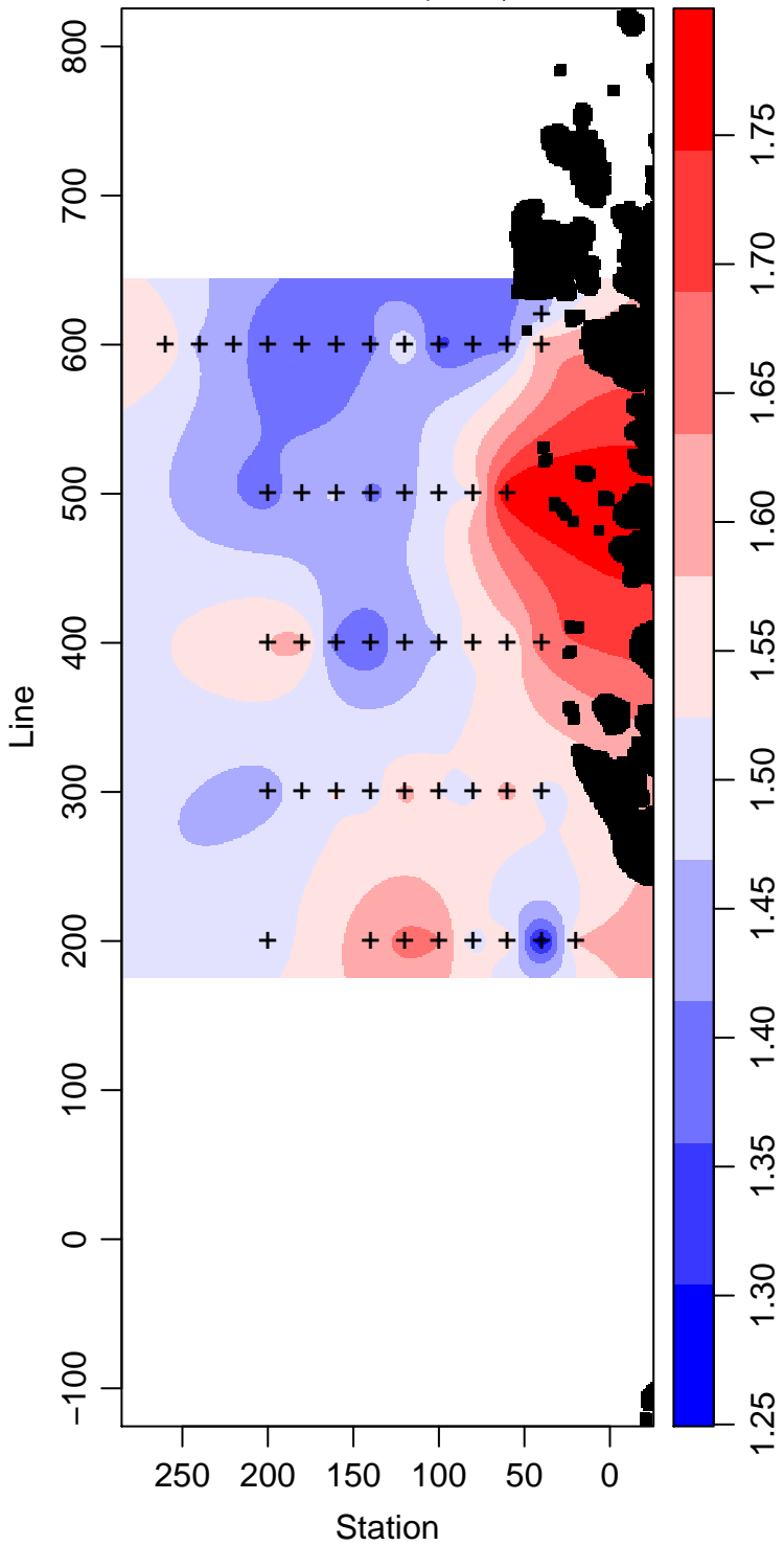
LMG04-01_45_Phosphate \mu\text{ mol L}^{-1}
