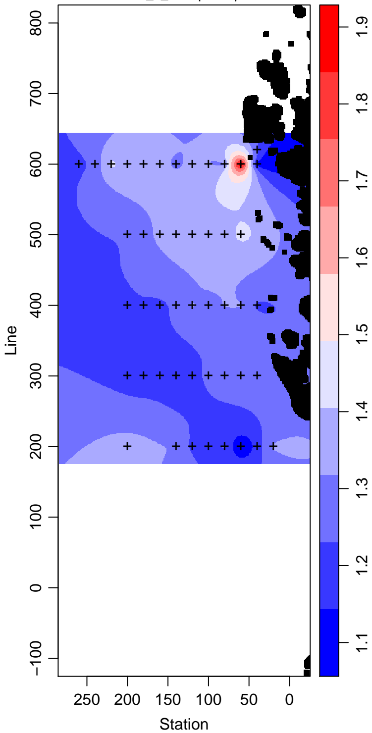
LMG04-01_5_Phosphate \mu\text{ mol L}^{-1}
