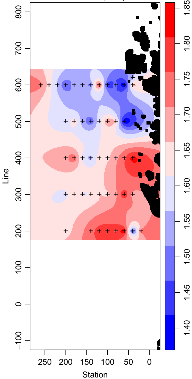
LMG04-01_65_Phosphate \mu\text{ mol L}^{-1}
