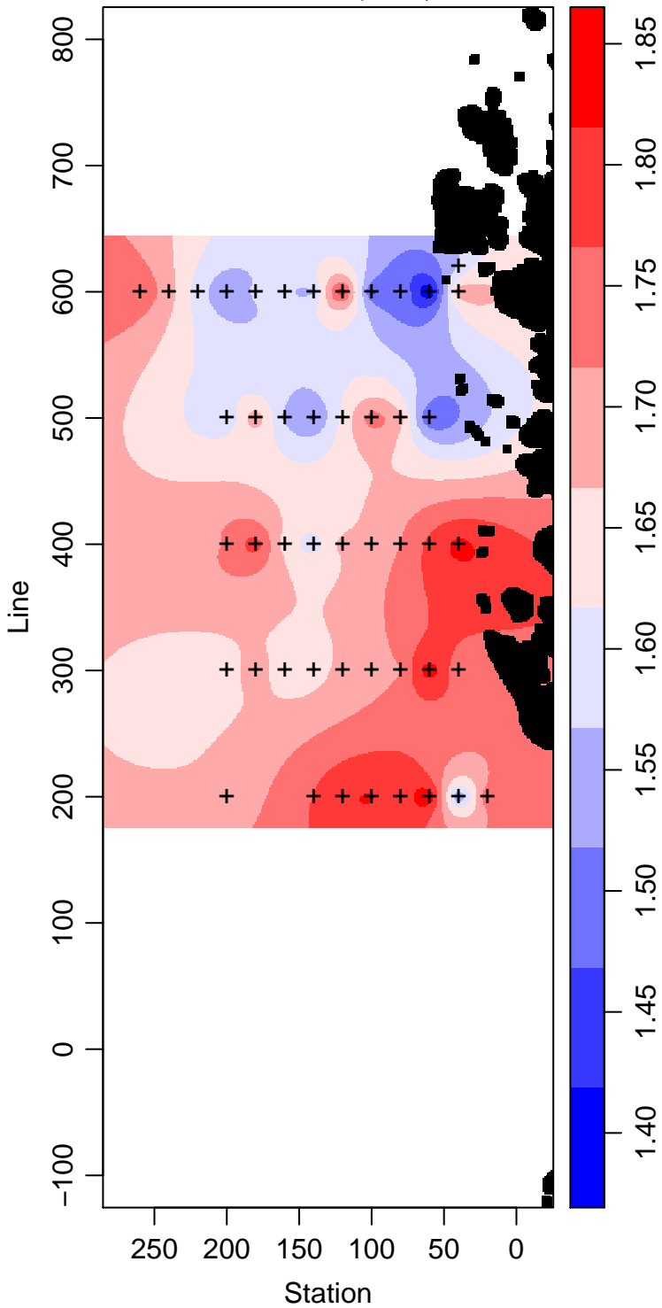
LMG04-01_70_Phosphate \mu\text{ mol L}^{-1}
