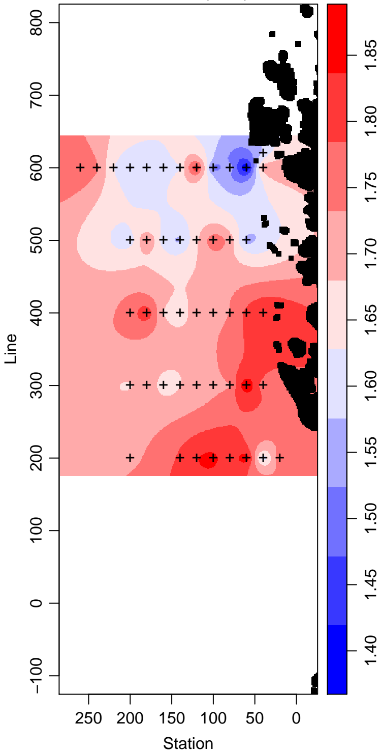
LMG04-01_75_Phosphate \mu\text{ mol L}^{-1}
