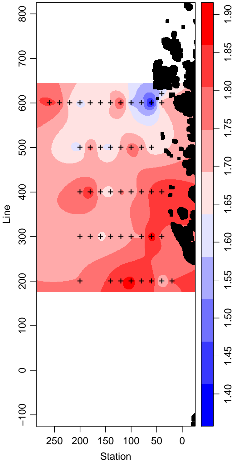
LMG04-01_80_Phosphate \mu\text{ mol L}^{-1}
