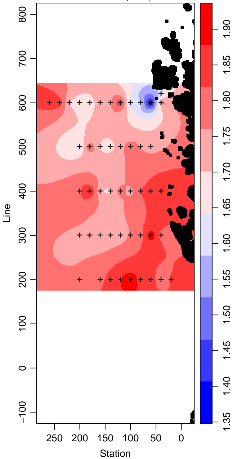
LMG04-01_85_Phosphate \mu\text{ mol L}^{-1}
