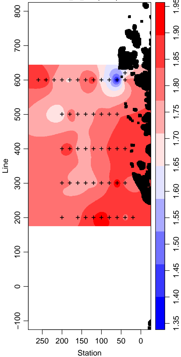
LMG04-01_90_Phosphate \mu\text{ mol L}^{-1}
