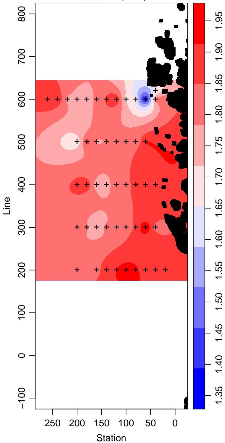
LMG04-01_95_Phosphate \mu\text{ mol L}^{-1}
