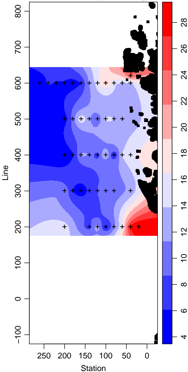
LMG04-01_15_Primary.Production mg m -3
