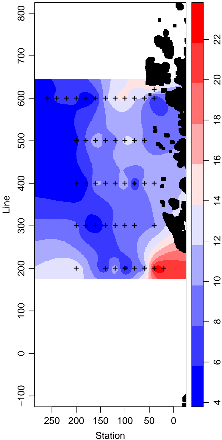
LMG04-01_20_Primary.Production mg m -3
