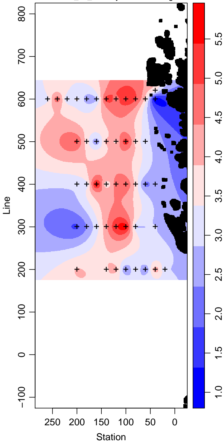
LMG04-01_45_Primary.Production mg m -3
