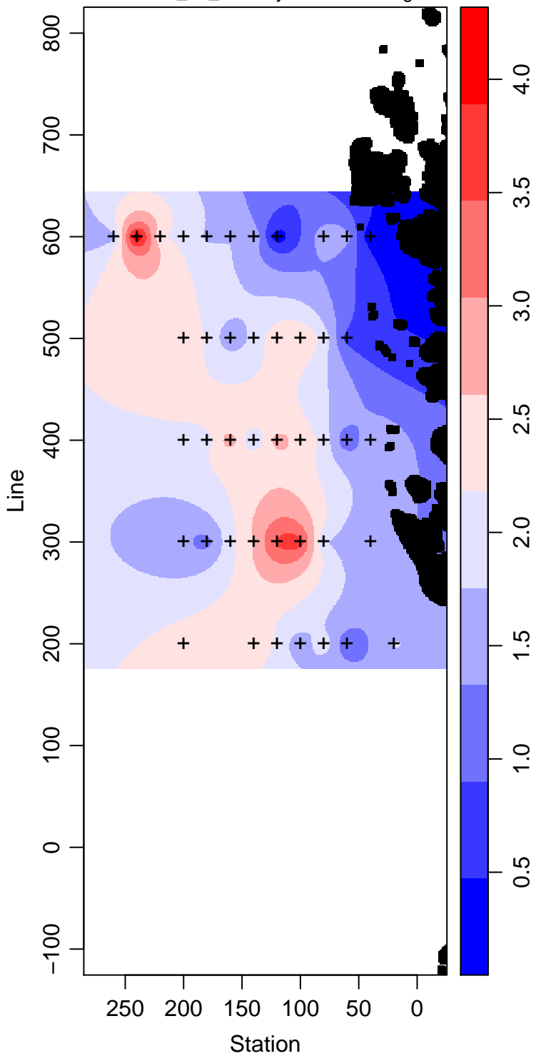
LMG04-01_60_Primary.Production mg m -3
