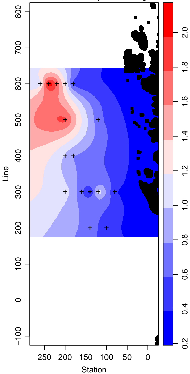
LMG04-01_80_Primary.Production mg m -3
